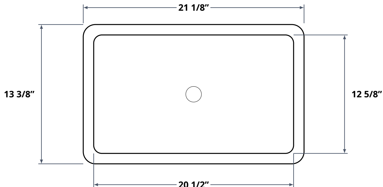
Top View
